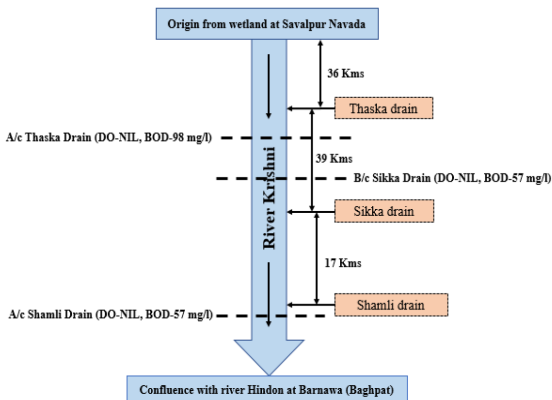
Figure 15 Flow diagram of river Krishni from origin to after confluence of Shamli drain
