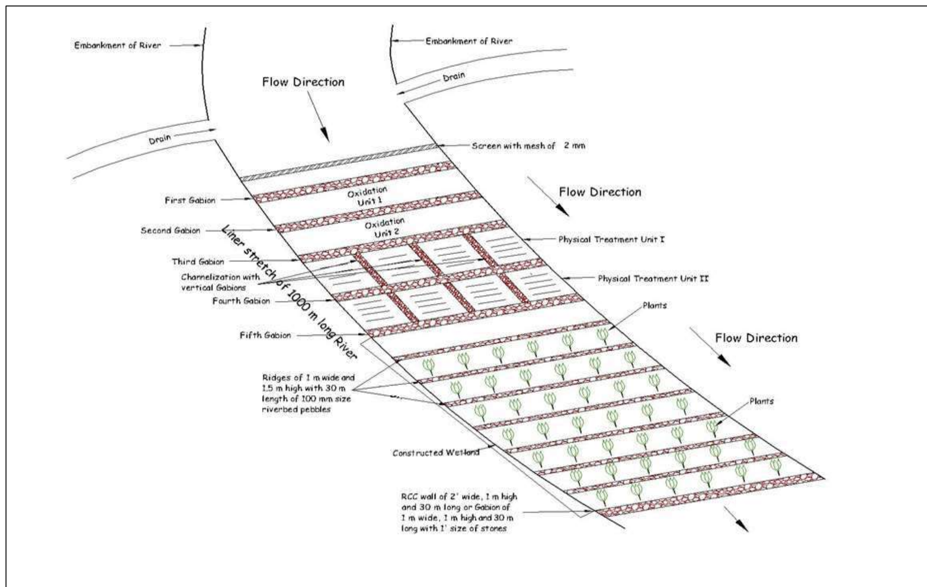
Schematic diagram of a Constructed Wetland System
